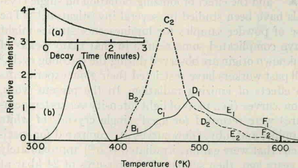
FIG. 2. Nonpressured sample: (a) Decay of light-induced luminescence, at 23°C, after 5-min exposure to mercury light, of an aged \alpha\text{-Al}_2\text{O}_3 crystal having in its history a 1-h exposure to a \text{Co}^{60} source, over 2 years ago. (b) Glow curve (solid line) obtained from the sample used in (a), and glow curve (dash) obtained from an aged sample not exposed to uv light. (The heating rate was about 50°/min.)
